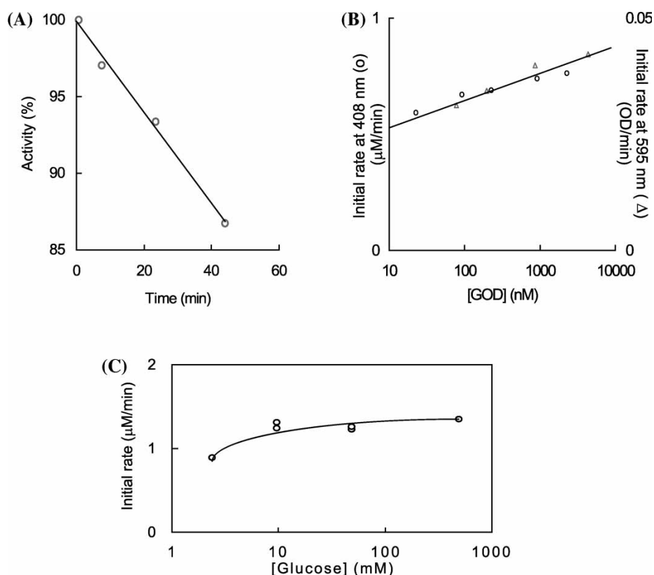
FIGURE 3 Dependence of initial rate of reaction on enzyme and glucose concentration. (A) Enzyme (42.2 \mu\text{M} ) was incubated with, cytochrome-c (18.2 \mu\text{M} ) and glucose (24.4 mM) at pH 3.9, and the activity of enzyme measured at times indicated. (B) Cytochrome-c (5.2 \mu\text{M} ) was mixed with glucose (49 mM) and reactions were started with enzyme at pH 2.9; the initial rate of the decrease in absorbancy at 408 nm and the increase in absorbancy at 595 nm was measured at different concentrations of enzyme. (C) Influence of glucose on reaction rates at 408 nm. The concentration of cytochrome-c was 8.45 \mu\text{M} and glucose oxidase was 0.198 \mu\text{M} , at pH 3.0.
