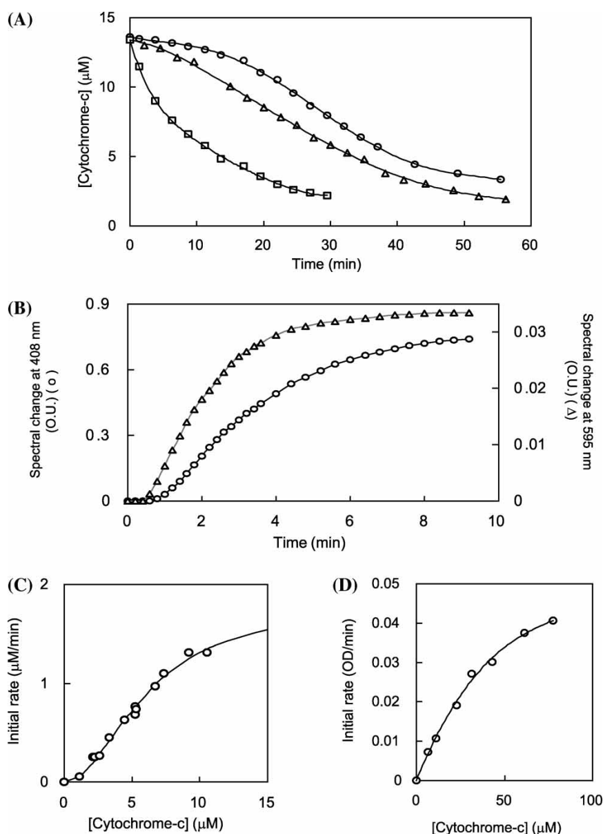
FIGURE 2 Influence of pH and substrate concentrations on spectral changes. (A) Influence of pH on the rate of spectral changes. Decrease in absorbancy of cytochrome-c ( 13.4\text{--}13.6\text{ }\mu\text{M} ) at 408\text{ nm} in the presence of glucose ( 41.5\text{ mM} ) and glucose oxidase ( 24.4\text{ nM} ), at pH 6.50 ( \circ ), pH 3.86 ( \Delta ) and pH 2.91 ( \square ). (B) Reaction progress curves at 408\text{ nm} and 595\text{ nm} , at pH 2.91. The spectral change of cytochrome-c ( 10.4\text{ }\mu\text{M} ) at 408\text{ nm} ( \circ ) and 595\text{ nm} ( \Delta ) in the presence of buffer, glucose ( 86\text{ mM} ), and glucose oxidase ( 86\text{ nM} ). Note that the spectral changes at 408\text{ nm} and 595\text{ nm} are in the opposite direction. (C) Dependence of initial rates of reaction at 408\text{ nm} on cytochrome-c concentration. Cytochrome-c was mixed with buffer, glucose ( 24\text{--}97\text{ mM} ) and the reaction was started with enzyme ( 1\text{--}10\text{ }\mu\text{M} ) at pH 2.9. The initial rate of decrease in absorbancy at 408\text{ nm} was measured at different concentrations of cytochrome. Other experimental details are given in text. (D) Dependence of initial rates of reaction at 595\text{ nm} on cytochrome-c concentration. Cytochrome-c was mixed with buffer, glucose ( 103\text{ mM} ) and glucose oxidase ( 105\text{ nM} ) at pH 2.9. The initial rate of increase in absorbancy at 595\text{ nm} was measured at different concentrations of cytochrome. Other experimental details are given in text.
