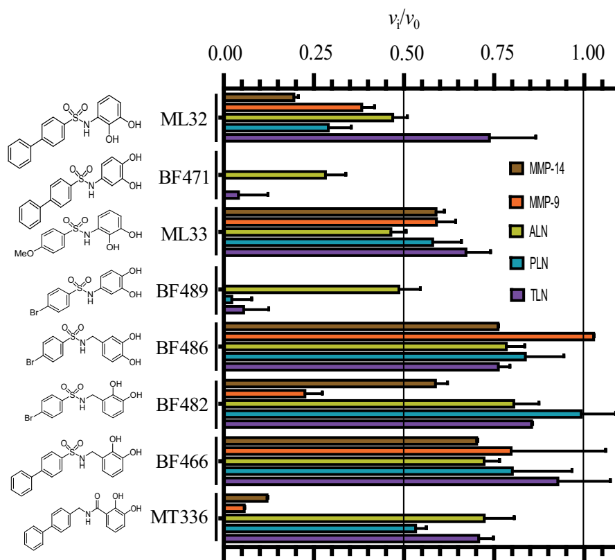
Figure 1. Inhibitory effect of 100 \mu M of the catechol containing compounds on the activity of the human metalloproteases, MMP-9 and MMP-14, and the bacterial metalloproteases TLN, PLN and ALN. The inhibition experiments were performed by using a fixed concentration of 4 \mu M of both the MMP-9 and MMP-14 substrate McaPLGL(Dpa)AR-NH 2 and the ALN, PLN and TLN substrate McaRPPGFSAFK(Dnp)-OH. The v_i/v_0 (mean \pm sd) were based on 4–6 experiments.
