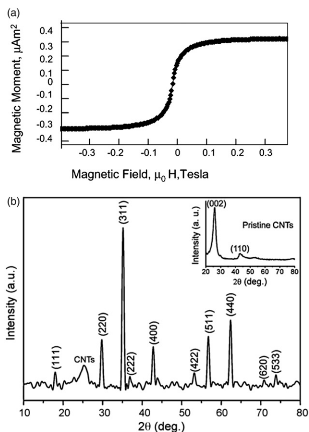
Figure 4. (a) Typical magnetization curve of a MCNT prepared by filling process [34]. (b) XRD pattern of CNTs/ \text{Fe}_3\text{O}_4 hybrids obtained by self-assembly method (the inset shows the XRD pattern of treated CNTs) [67].
