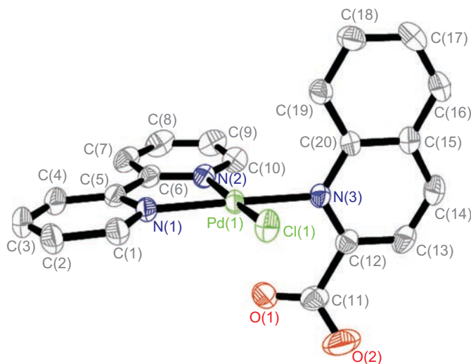
Figure 2. Independent molecule of complex 1 with numbering of atoms (four crystal water and H atoms are omitted for clarity) at 30% probability thermal ellipsoids.
