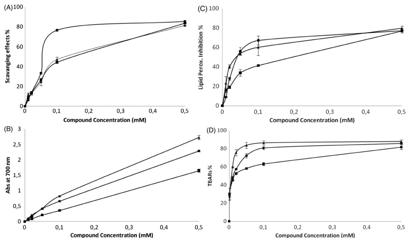
Figure 3. (A) Scavenging activity on DPPH radicals (RSA), (B) RP (Abs at 690 \text{ nm} ), (C) CLS and (D) TBARS assay using brain homogenized tissue for compounds 3a–c ( 3a \blacktriangle ; 3b \blacksquare ; 3c \bullet ). Results are the mean \pm SD of three independent experiments.
