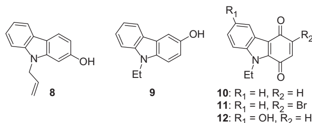
Figure 2. Structures of tricyclic hydroxycarbazole and carbazolequinone derivatives 8–12 .
