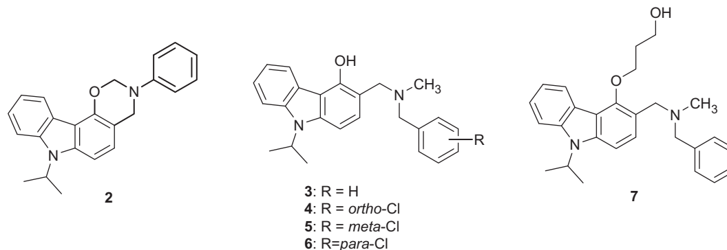
Figure 1. Structures of oxazinocarbazole 2 and aminomethylated carbazoles 3–7 .
