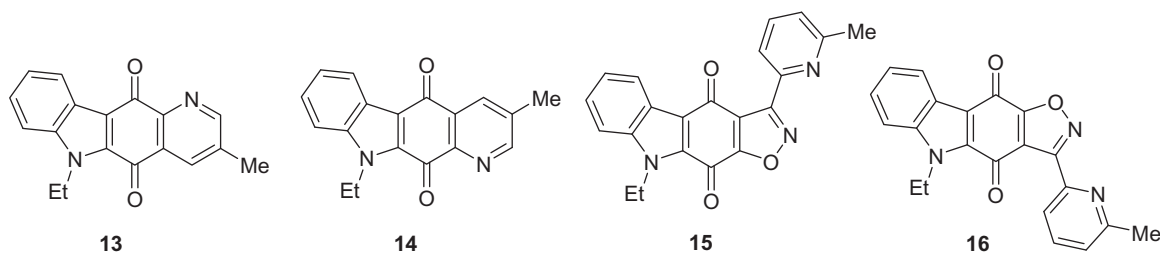
Figure 3. Structures of pyrido and isoxazolocarbazolediones 13–16 .
