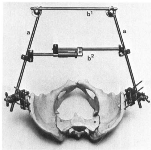
Figure 1. The trapezoid compression frame is anchored to the two iliac crests with three pins on each side. The vertical bars (a) are connected with a horizontal upper bar (b 1 ). The compression bar (b 2 ) is placed midway between the upper bar and the anchorage to the iliac crest. Compression conveys the compressive force to the posterior, weight-bearing arch of the pelvic girdle (from Slätis & Karaharju Clin. Orthop. 1980, 151, p. 75, Figure 1).
